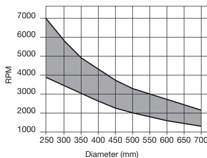
Minimum and maximum RPM based on the blade diameter.
