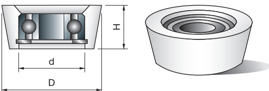
Conical rub collars for ball bearing.
